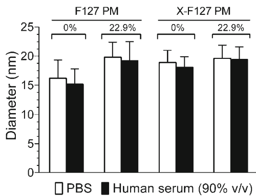
Fig. 6 Effect of peripherally cross-linking the shell of F127 PM on the hydrodynamic diameter in human serum. F127 polymer micelles alone (F127 PM) or individually cross-linked with ED at 76% of total PEO blocks (X-F127 PM) were loaded with CA4 at 22.9 wt% as described in Fig. 5. Lyophilized formulations were resuspended in PBS, diluted to 2 mg/mL in PBS (open bars) or human serum (90% v/v) (closed bars), and incubated at 37°C for 24 h. Average hydrodynamic diameters \pm SD ( n=3 independent samples from same batch) were then determined by DLS and compared by one way ANOVA with Tukey's post-test. The polydispersity index of the samples ranged from 0.143 to 0.269 and larger peaks indicative of PM aggregation were not observed (data not shown).
